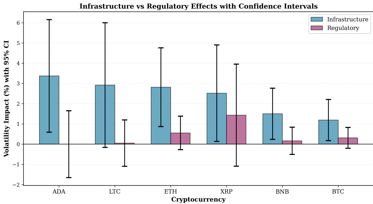
Figure 4: Infrastructure vs Regulatory Effects with 95% Confidence Intervals
